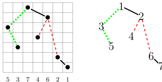
Figure 1: The t-shelf corresponding to the permutation 5 3 7 4 6 2 1; dotted (dashed) lines correspond to an occurrence of the third (fourth) pattern in the set \mathcal{B}_3 listed above.
