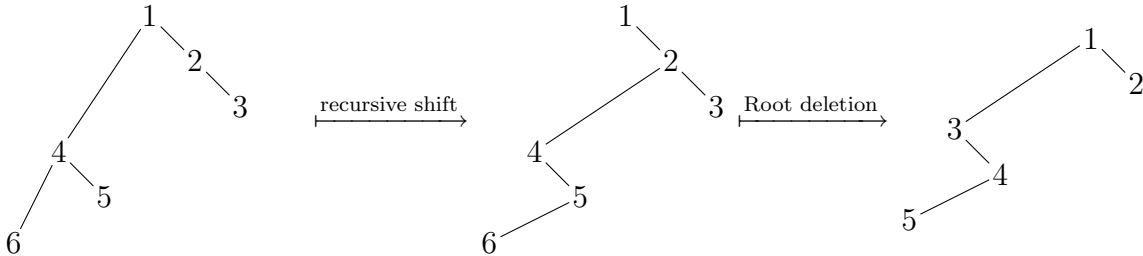
Figure 6: An unordered binary increasing tree in standard representation and its image after the recursive shift process, and after the deletion of the root.
