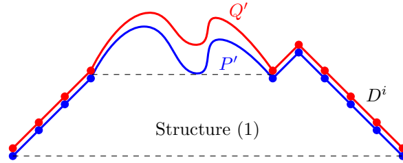
Figure 3: The structure of linear intervals [P, Q] in \mathbb{F}_n^p when \text{type}(P) = \text{type}(Q) . See Lemma 1
