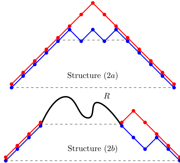
Figure 4: The structure of linear intervals [P, Q] in \mathbb{F}_n^p when \text{type}(Q) \geq \text{type}(P) + 2 . See Lemma 2
