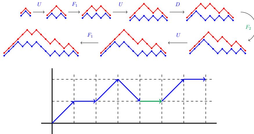
Figure 6: The generation of the interval [U^2(UD)^3D^2(UD)^3, U^4(UD)^2D^2(UD^2)^2] using the rules in the proof of Theorem 6. This interval is thus associated with the bicolored Motzkin prefix UF_1UDF_2UF_1 .
