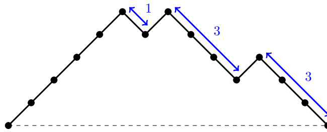
Figure 9: The path P = U^5D(UD^3)^2 \in \mathcal{F}_7^\infty is associated with the composition \lambda(P) = (3, 3, 1) .
