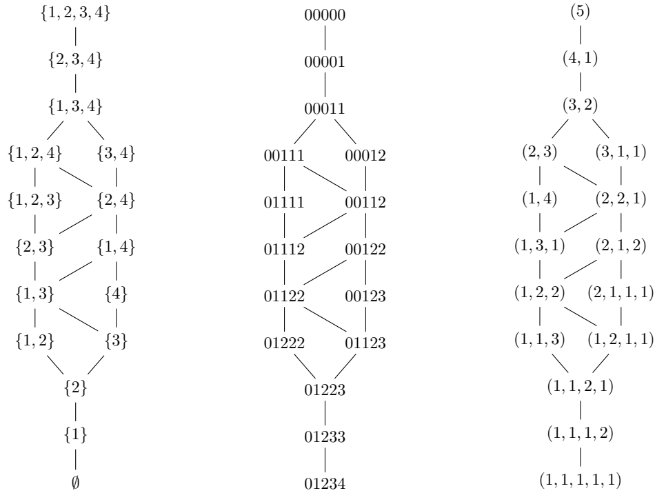
Figure 12: The lattice \mathbb{F}_5^\infty on the power set of \{1, 2, 3, 4\} (left), the non-decreasing Catalan words of length 5 (center), and the compositions of 5 (right).
