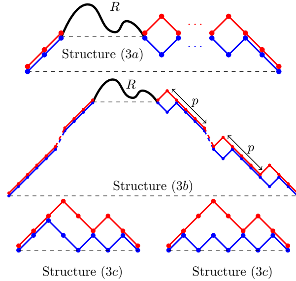
Figure 5: The structure of linear intervals [P, Q] in \mathbb{F}_n^p when \text{type}(Q) = \text{type}(P) + 1 . See Lemma 3
