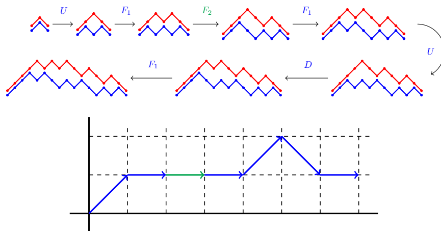
Figure 7: The generation of the interval [U^2(UD)^2(DU)^2D^2(UD)^2, U^3(UD)^2(UD^2)^3] using the rules in the proof on Theorem 8. This interval is thus associated with the bicolored Motzkin prefix UF_1F_2F_1UDF_1 .
