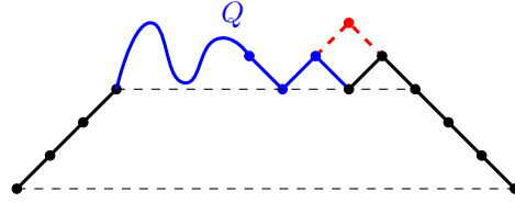
Figure 2: Illustration of Subcase 1(a) in the proof of Theorem 1. The last valley of P cannot produce a covering because this would create an occurrence DUU .
