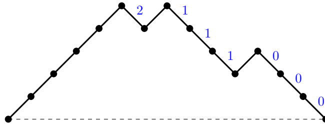
Figure 8: The path P = U^5 D (UD^3)^2 \in \mathcal{F}_7^\infty is associated with the Catalan word \omega(P) = 0001112 .
