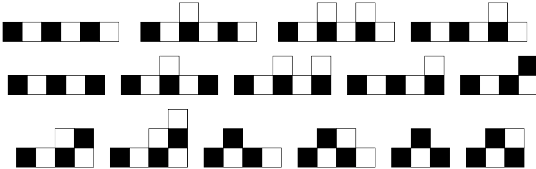
FIGURE 8. The 15 Catalan polyominoes P with \text{black}(P) = 3 .
