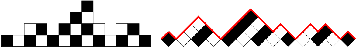
FIGURE 6. The black cell capacity of a Catalan polyomino is interpreted via Dyck paths.
