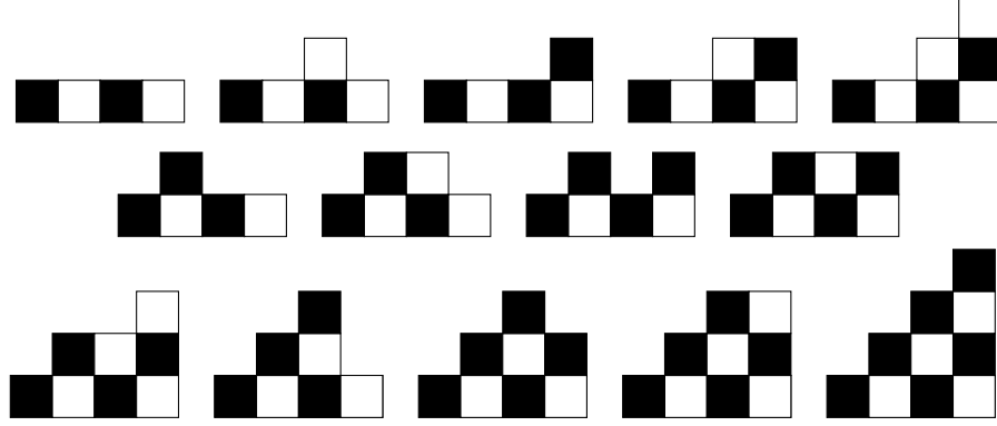
FIGURE 5. The 14 Catalan polyominoes of length 4. There are 2 (resp 5, 4,2,1) polyominoes with black cell capacity 2 (resp. 3,4,5,6).
