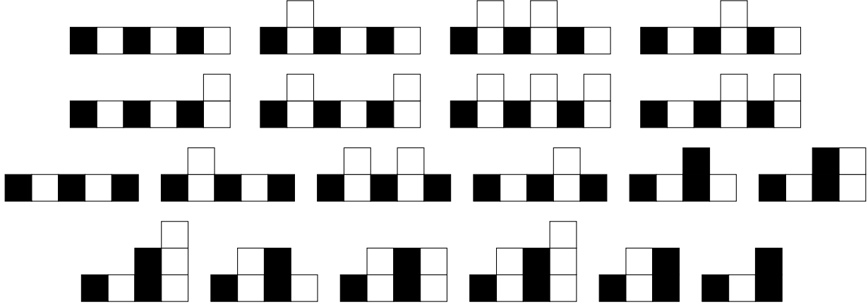
FIGURE 9. The 20 Catalan polyominoes P with \text{verblack}(P) = 3 .
