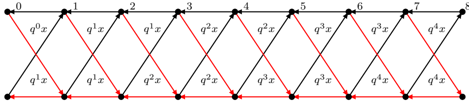
FIGURE 7. Graph (automaton) to recognize partial Dyck paths with respect to the length (marked with x ) and the black cell capacity (marked with q ).
