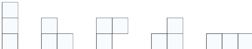
FIGURE 7. The directed animals of size 3.
