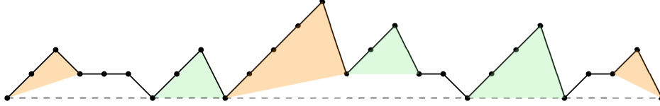
FIGURE 1. Symmetric and asymmetric peaks of a MAP1.
