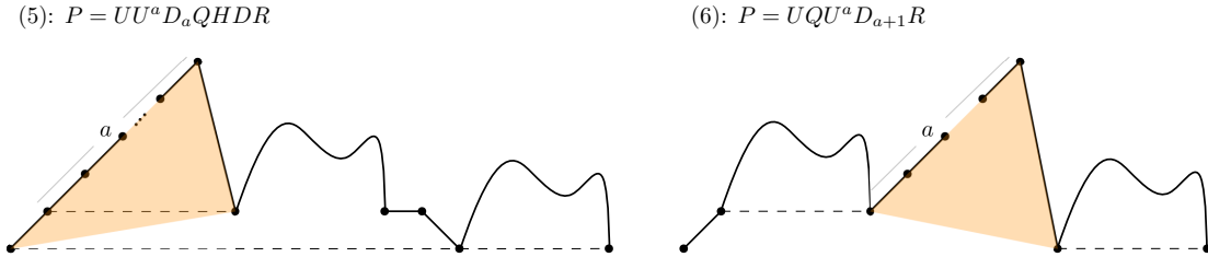
FIGURE 3. Decomposition of cases (5) and (6).
