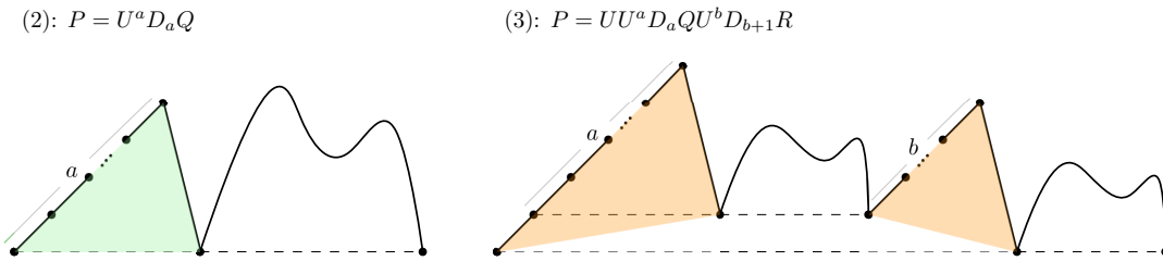
FIGURE 2. Decomposition of cases (2) and (3).
