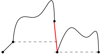
FIGURE 4. Decomposition of cases (7) and (8).
