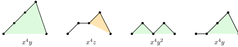
FIGURE 6. The MAP2 of length 4 and their contribution in M'_{sp,ap}(x, y, z) .
