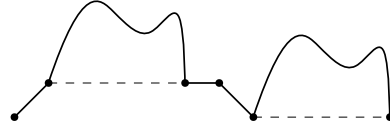
FIGURE 4. Decomposition of cases (7) and (8).
