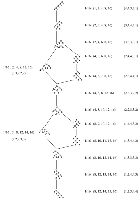
Fig. 2. The pruning-grafting lattice B_4 . Each tree is encoded with its feasible and distribution sequences.
