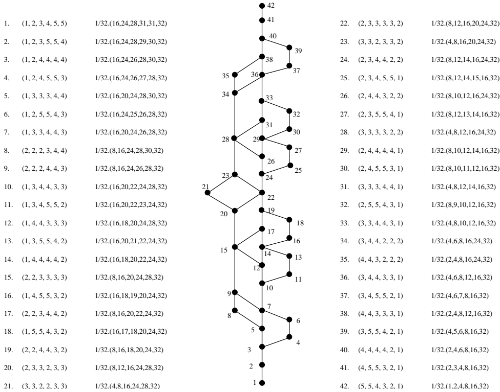
Fig. 3. The pruning-grafting lattice B_5 . Each tree is encoded with its feasible and distribution sequences.
