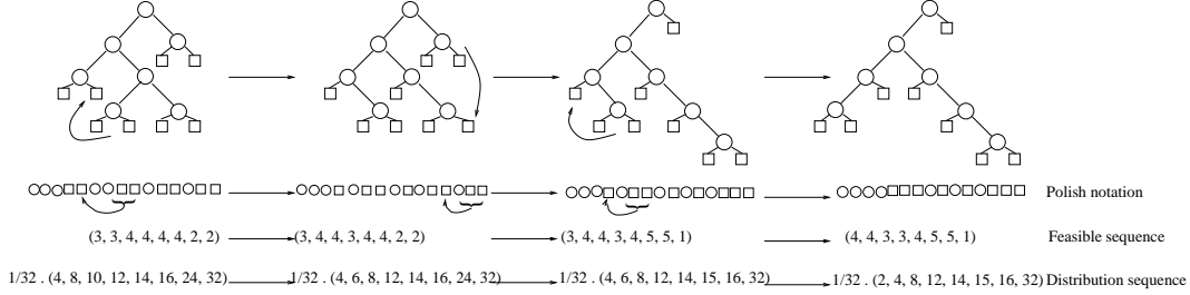
Fig. 1. Three pruning-grafting transformations in B_7 .
