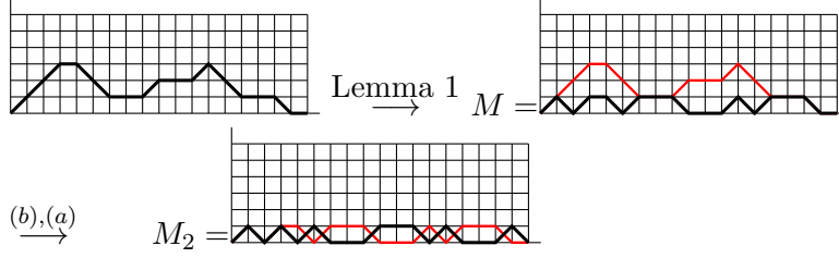
Figure 8: Illustration of the example in the proof of Lemma 8.
