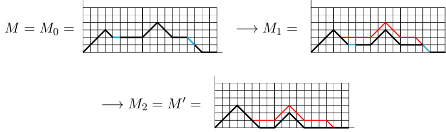
Figure 3: Illustration of the example described in the proof of Lemma 2.
