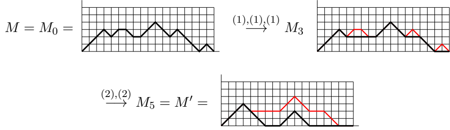
Figure 4: Illustration of the example described in the proof of Lemma 3.
