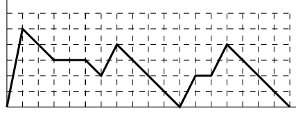
Figure 1: A Lukasiewicz path of length 18: U_5DDFFDU_2DDDDU_2FU_2DDDD .
