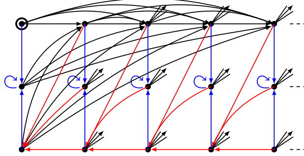
Figure 3: The state diagram for the generation of partial Lukasiewicz paths. Black (resp. red, blue) arrows corresponds to up-steps (resp. down-steps, horizontal steps).
