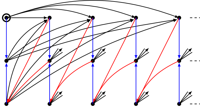
Figure 4: The state diagram for partial alternate Łukasiewicz paths. Black (resp. red, blue) arrows corresponds to up-steps (resp. down-steps, horizontal steps).
