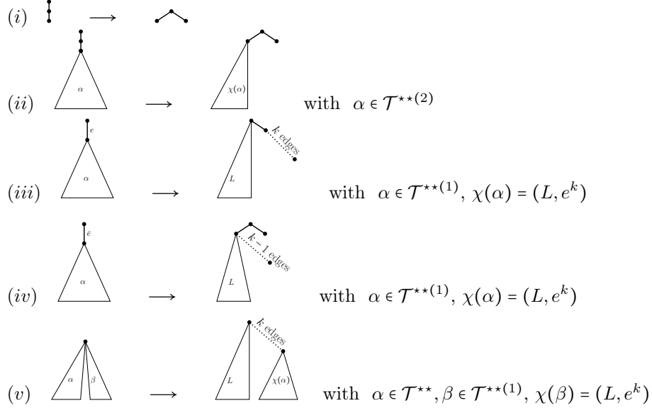
Figure 6: An illustration of the bijection \chi .
