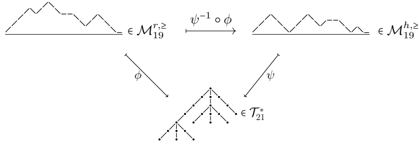
Figure 5: Example of one-to-one correspondence between two Motzkin paths in \mathcal{M}_{19}^{r, \ge} and \mathcal{M}_{19}^{h, \ge} passing by a tree in \mathcal{T}_{21}^* .
